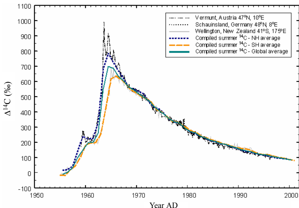
Figure 9 Compiled summer hemispheric and global ^{14}\text{C} curves versus atmospheric ^{14}\text{C} records for Vermunt and Schauinsland (central Europe; Levin et al. 1994) and Wellington (New Zealand; Manning and Melhuish 1994). The compiled data sets are presented in Tables 5a–b, 6a–b, and 7.
