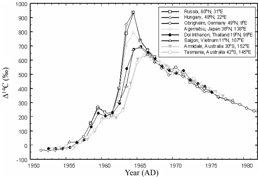
Figure 2 ^{14}\text{C} in tree rings at different locations. Data sources are Kolesnikov et al. (1970) for Russia, Hertelendi and Csongor (1982) for Hungary, Levin et al. (1985) for Obrigheim (Germany), Muraki et al. (1998) for Agematsu (Japan), Kikata et al. (1992, 1993) for Saigon (Vietnam), Hua et al. (2000) for Doi Inthanon (Thailand) and Tasmania (Australia), and Hua et al. (2003) for Armidale (Australia).
