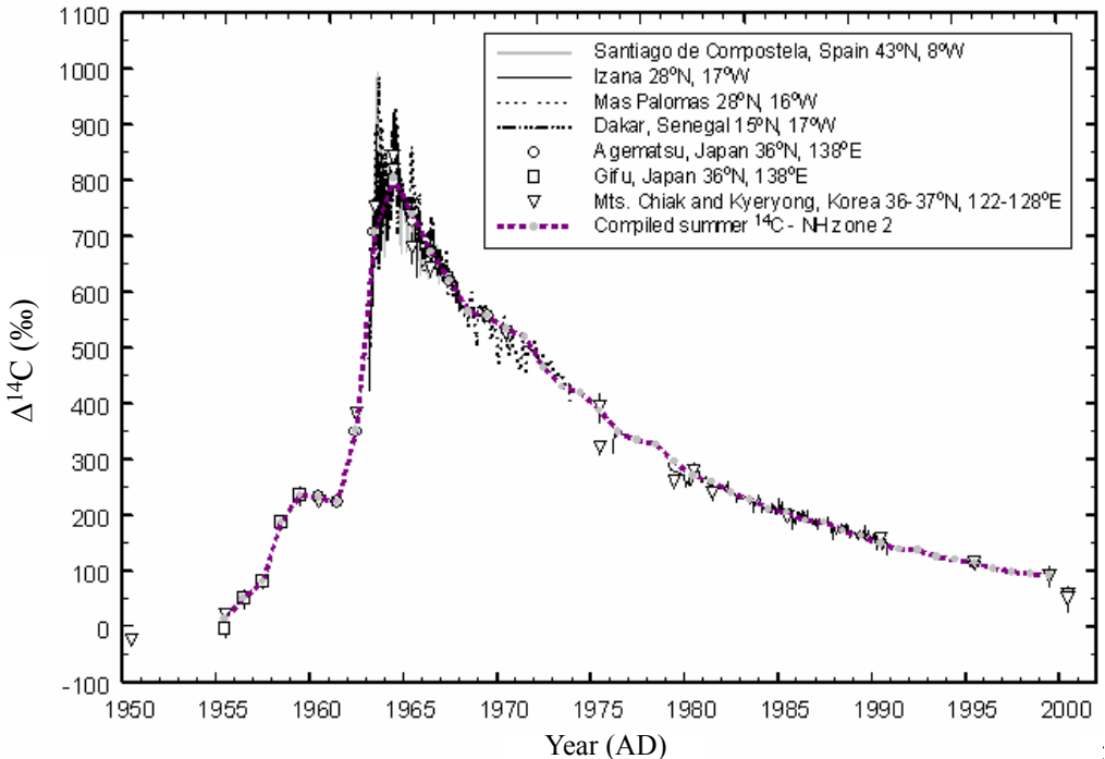
Figure 5 Compiled summer atmospheric ^{14}\text{C} curve for NH zone 2 versus atmospheric ^{14}\text{C} records (lines) and tree-ring ^{14}\text{C} data (symbols) available for the zone. Data sources are given in Tables 4b and 5b.
